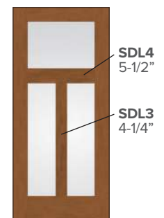
SDL5 Some door styles use a combination of 4-1/4" and 5-1/2" divider bars.
