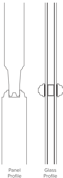
Performance 1-3/8" SDL Bar, 1-7/16" Double Hip Raised Panel with IG Glass
