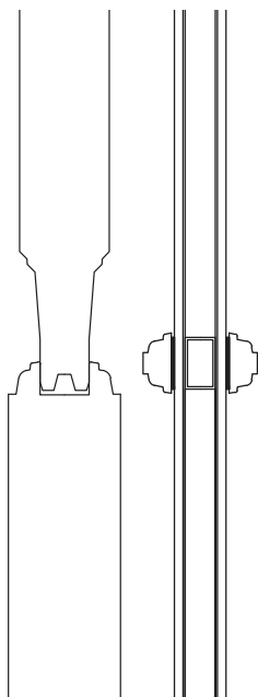
Panel Profile
