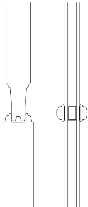
Panel Profile
