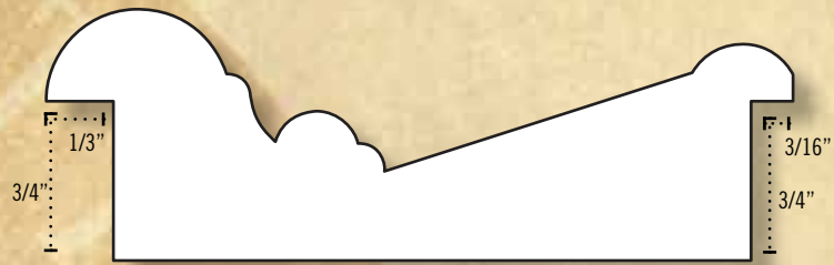
PLP312 1-3/16 x 3-1/2 Page 25
