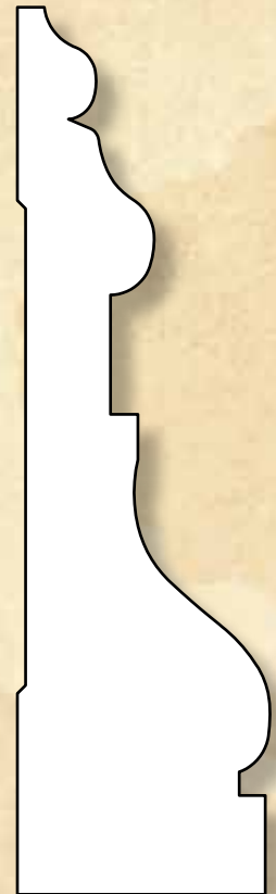
GS425 MDF 1-3/16 x 4-1/4 Page 14
