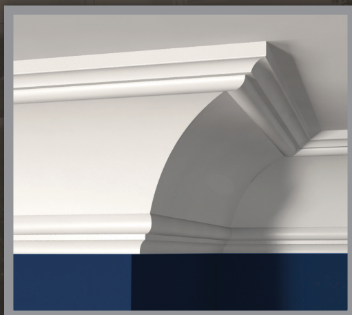
DCR734 1-21/32" x 7-3/4" 18' Lengths
